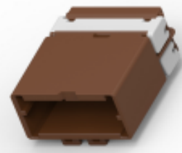
TE Part # 1123353-3 040 MLC CAP HSG ASSY 16P
